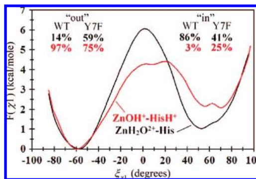
Figure 7. Free energy profile (PMF) for the rotation of His64 about the \chi_1 dihedral angle in the ZnH 2 O 2+ -His system (black) and the ZnOH + -HisH + system (red) for the Y7F mutant of HCA II. The subset percentages correspond to the "in" and "out" percentages as determined by integrating F(\xi_{\chi_1}) for both the WT (curves not shown, from ref 12) and the Y7F mutant.
