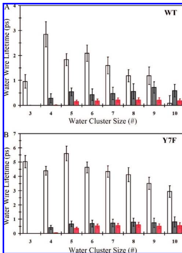
Figure 3. Water wire lifetimes for the continuous hydrogen bonded water wire that connects the zinc-bound water/hydroxide and the protonated/unprotonated \text{N}_\delta of His64. (A) Water wire lifetime distribution for WT- \text{ZnH}_2\text{O}^{2+} -His in the “in” orientation (black no fill), WT- \text{ZnH}_2\text{O}^{2+} -His in the “out” orientation (black with black fill), WT- \text{ZnOH}^+ -HisH + in the “out” orientation (red with red fill). (B) Water wire lifetime distribution for Y7F- \text{ZnH}_2\text{O}^{2+} -His in the “in” orientation (black no fill), Y7F- \text{ZnH}_2\text{O}^{2+} -His in the “out” orientation (black with black fill), Y7F- \text{ZnOH}^+ -HisH + in the “out” orientation (red with red fill).
